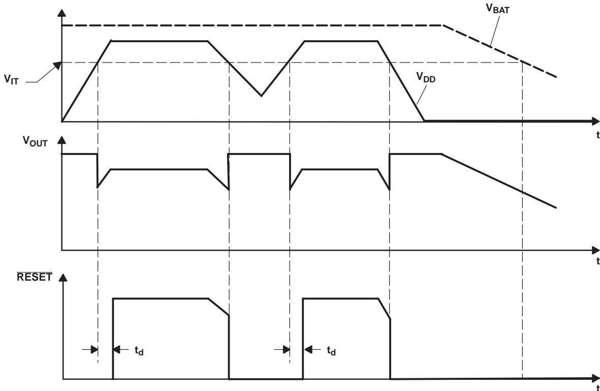
Timing Diagram
